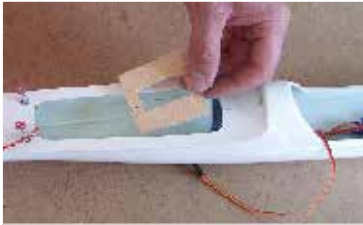
147. ... desku vlepíme do trupu... ... glue servo plate to the fuselage ...
